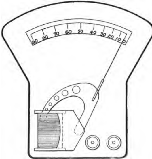
FIG. 421. —Constructional Diagram of one type of Ampere-Meter, or Ammeter. This particular instrument represents the variety known as the solenoid ammeter. It operates as follows: A hollow coil of wire, or solenoid, is connected to the terminals of the circuit, so that the current passes through it. The effect of the passing current is to attract the pivoted iron bar, on one end of which the dial needle is carried. According to the strength of the current passing through the coil the bar is more or less drawn into the eye of the coil. Thus the needle is able to register the amperage on the circuit, according to the determined relation between the conductivity of the wire and the strength of the current passing. The pivoted arm is arranged to be withdrawn from the coil when the amperage of the current falls, either by gravity or a suitably arranged tension spring. Other ammeters are constructed on principles differing from the one shown.
